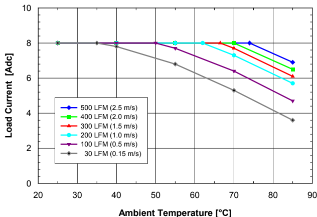
Fig. 6.0V.1: Available load current vs. ambient air temperature and airflow rates for SQ48T08060 converter with D height pins mounted vertically with V_{in} = 48\text{V} , air flowing from pin 3 to pin 1, and maximum FET temperature \leq 120^\circ\text{C} .
