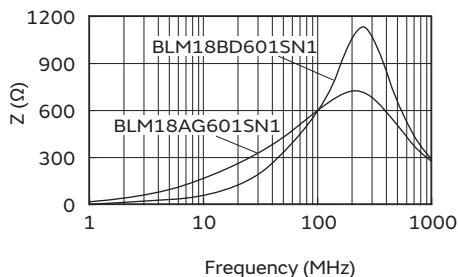
Comparison of Impedance Curve
