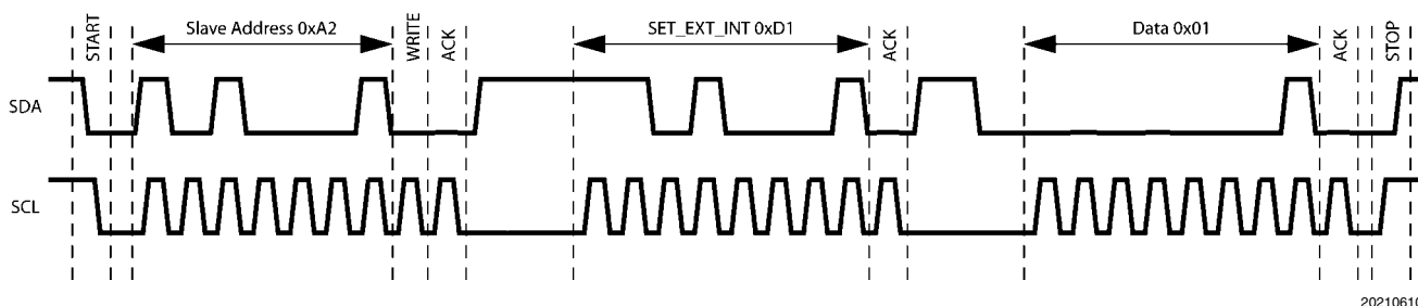
FIGURE 8. Host Write Command
