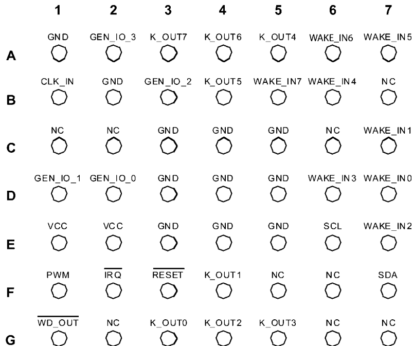
Top View — MICRO-ARRAY Package See NS Package Number GRA49A
