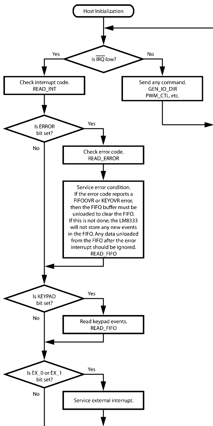
FIGURE 11. Interrupt Processing
