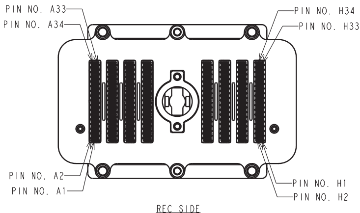
Rear View
