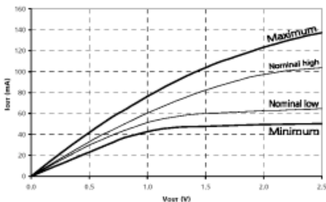
Figure 9: Pull-Down Characteristics
