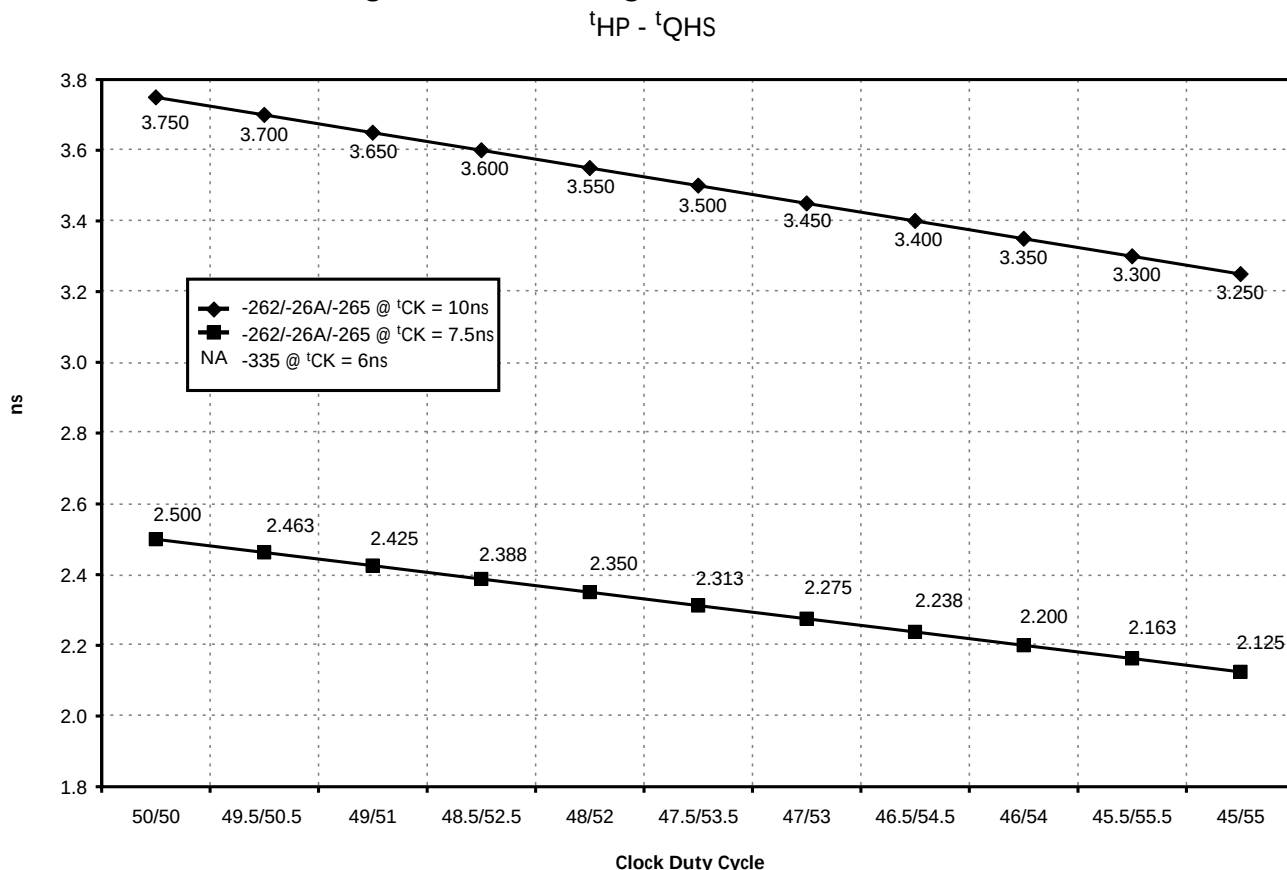
Figure 8: Derating Data Valid Window
