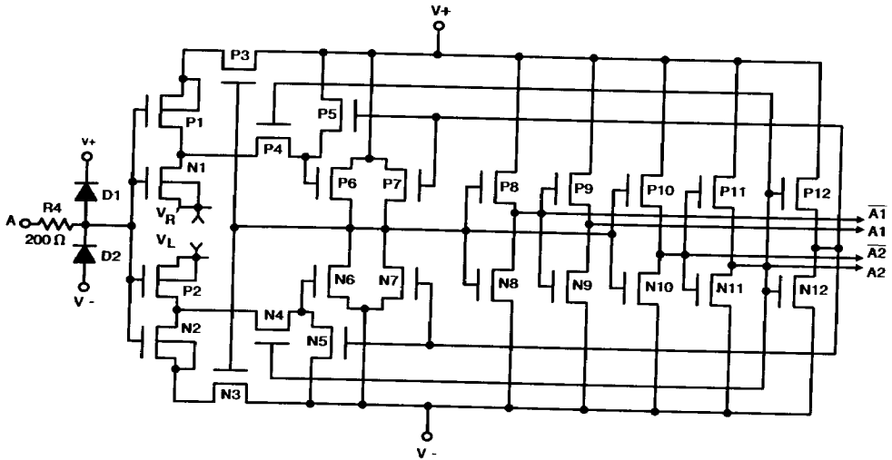
DIGITAL INPUT BUFFER AND LEVEL SHIFTER
