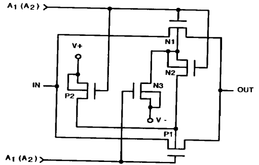
SWITCH CELL
