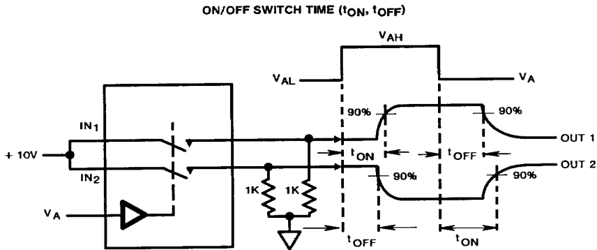
SWITCHING TIMES FOR POSITIVE DIGITAL TRANSITION
