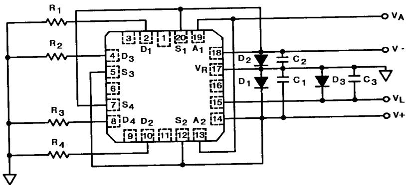
HI-5045/883 HI-5049/883 CERAMIC LCC
