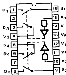
HI-50XX/883 (CERAMIC DIP)
