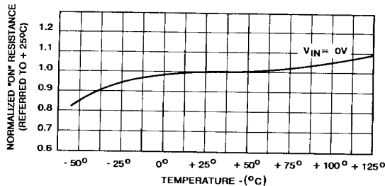
NORMALIZED "ON" RESISTANCE vs. TEMPERATURE
