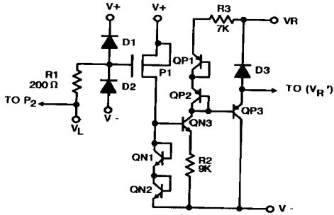
TTL/CMOS REFERENCE CIRCUIT *
