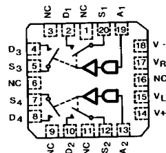
HI4-50XX/883 (CERAMIC LCC)
