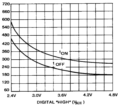
SWITCHING TIMES FOR POSITIVE DIGITAL TRANSITION
