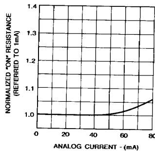
NORMALIZED "ON" RESISTANCE vs. ANALOG CURRENT
