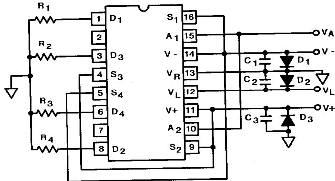
HI-5045/883 HI-5049/883 CERAMIC DIP
