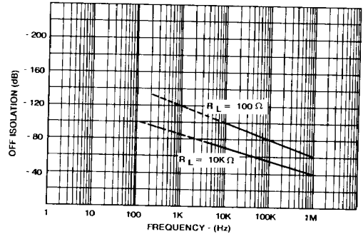
"OFF" ISOLATION vs. FREQUENCY
