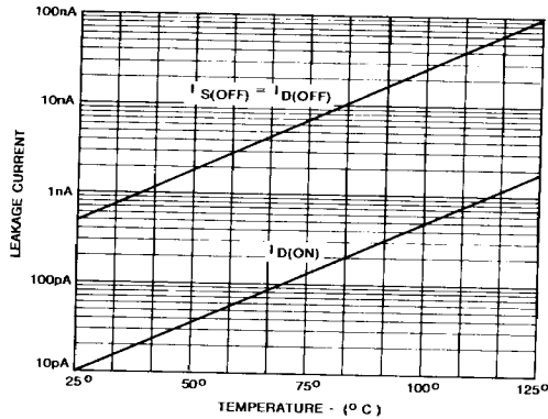
ON/OFF LEAKAGE CURRENT vs. TEMPERATURE
