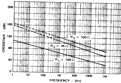
CROSSTALK vs. FREQUENCY
