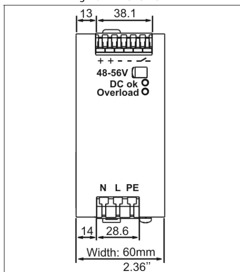
Fig. 20-1 Front view
