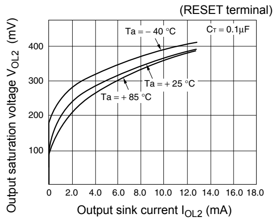
Output saturation voltage vs. Output sink current
