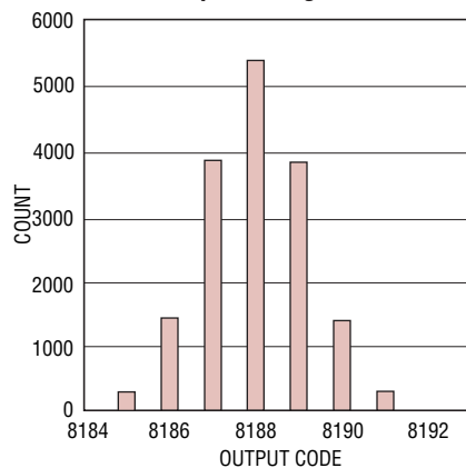
LTC2266-14: Shorted Input Histogram
