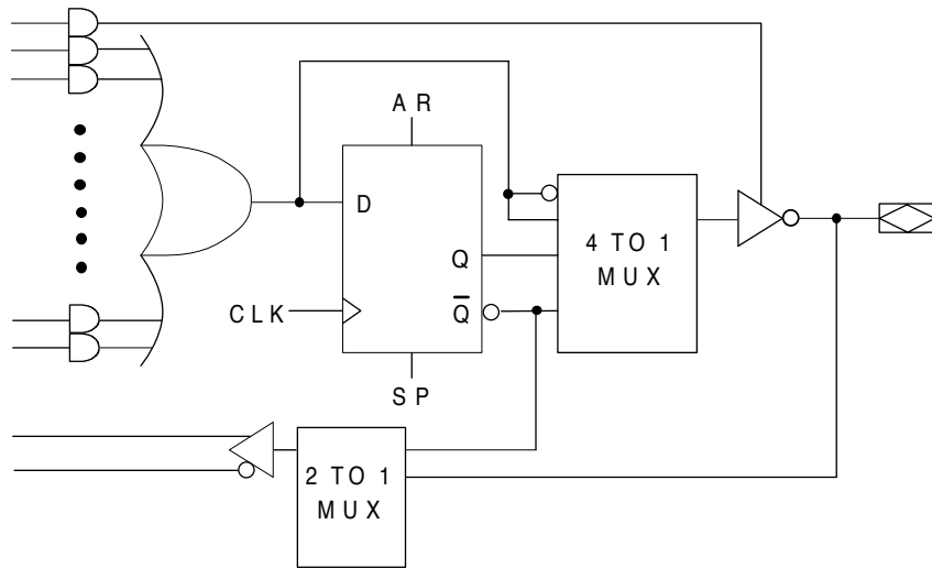
GAL26CV12 OUTPUT LOGIC MACROCELL (OLMC)
