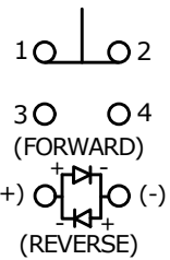
SPDT LED SCHEMATIC
