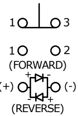
SPDT LED SCHEMATIC
