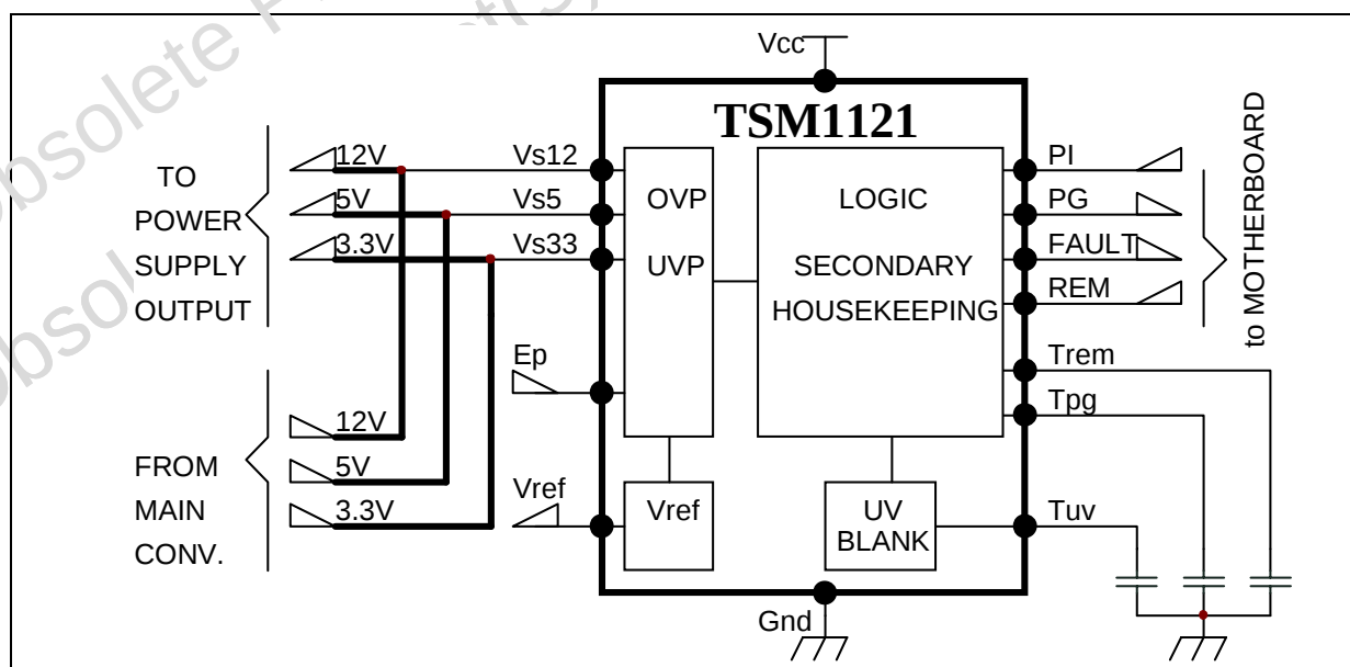
Fig. 2: Internal Schematic
