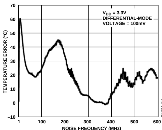
Figure 38. External Temperature Error vs. Differential-Mode Noise Frequency
