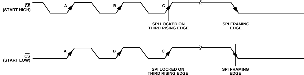
Figure 59. Serial Interface—Selecting and Locking SPI Protocol
