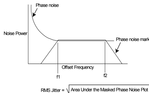
Figure 6. RMS Phase Jitter
