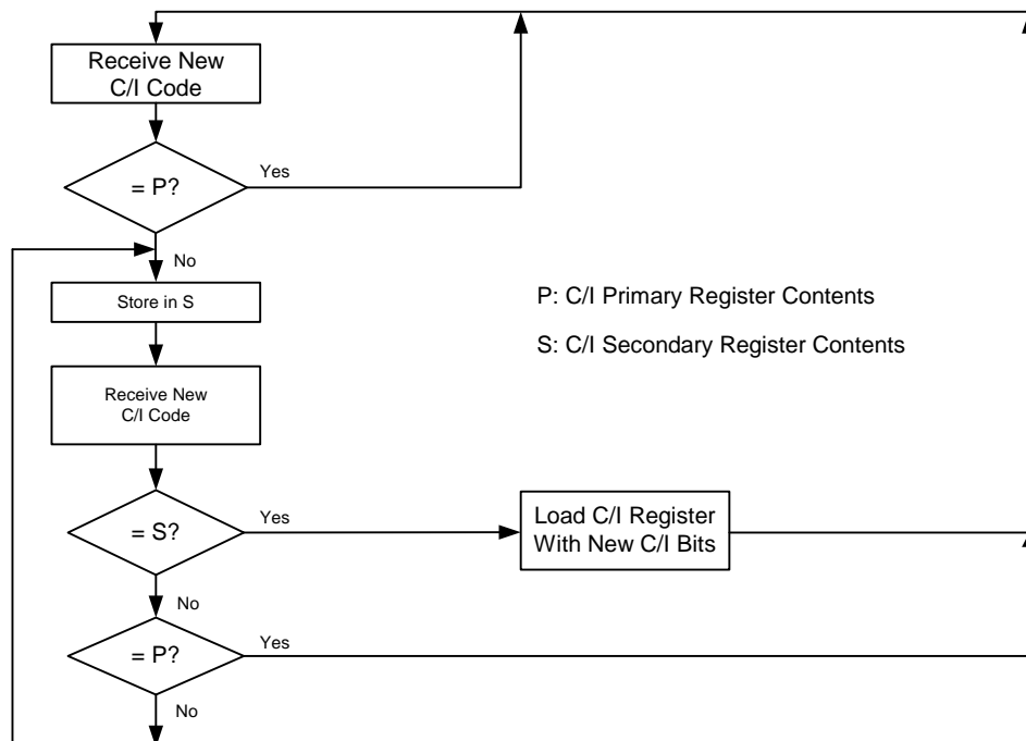
Figure 63. Protocol for Receiving C/I Bits in the Dual ProSLIC
