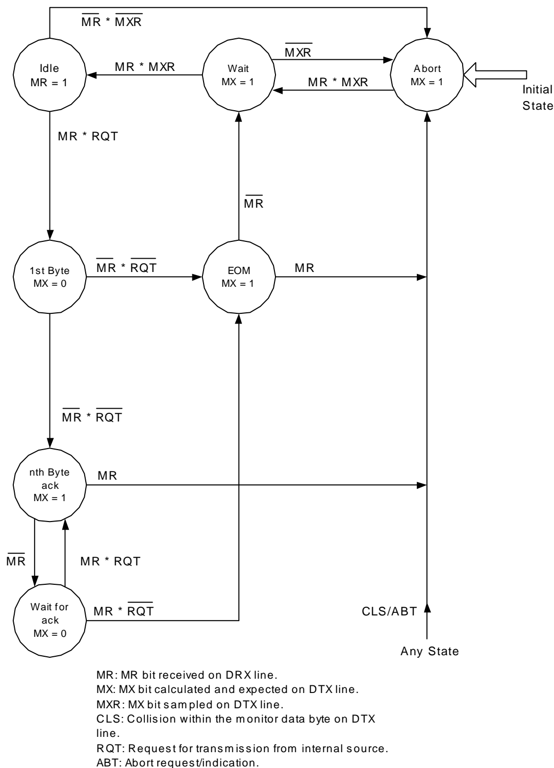
Figure 59. Dual ProSLIC Monitor Transmitter State Diagram
