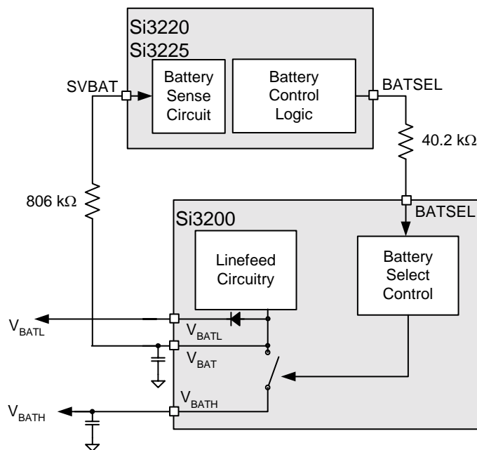
Figure 22. External Battery Switching Using the Si3220/Si3225
