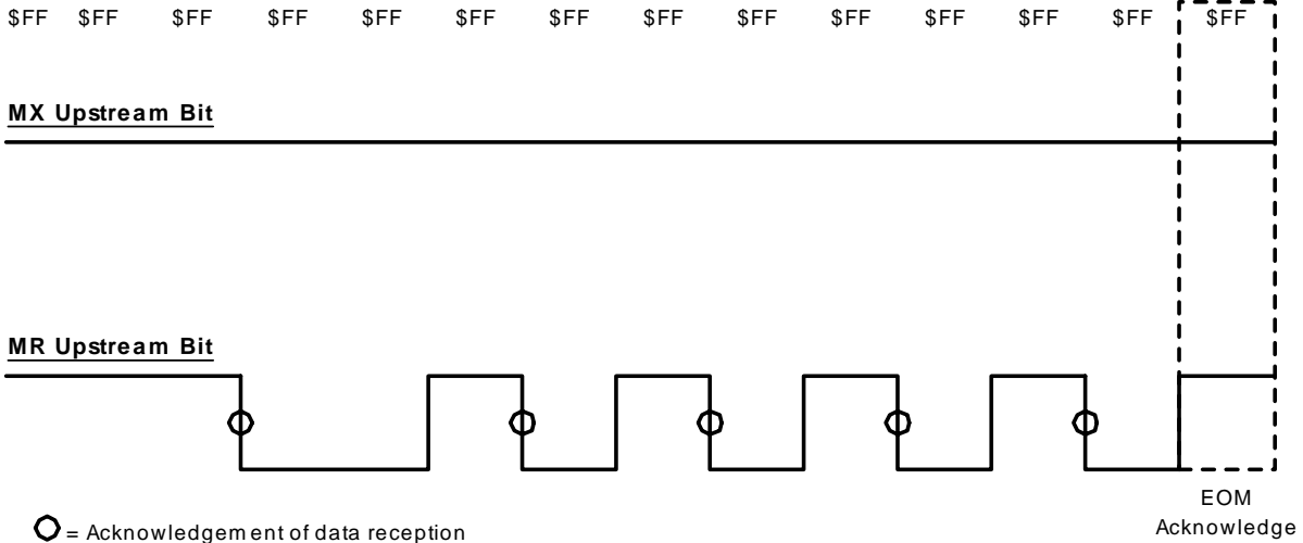
Figure 61. Example Write to Registers $10 and $11 in Channel 0 of the Dual ProSLIC
