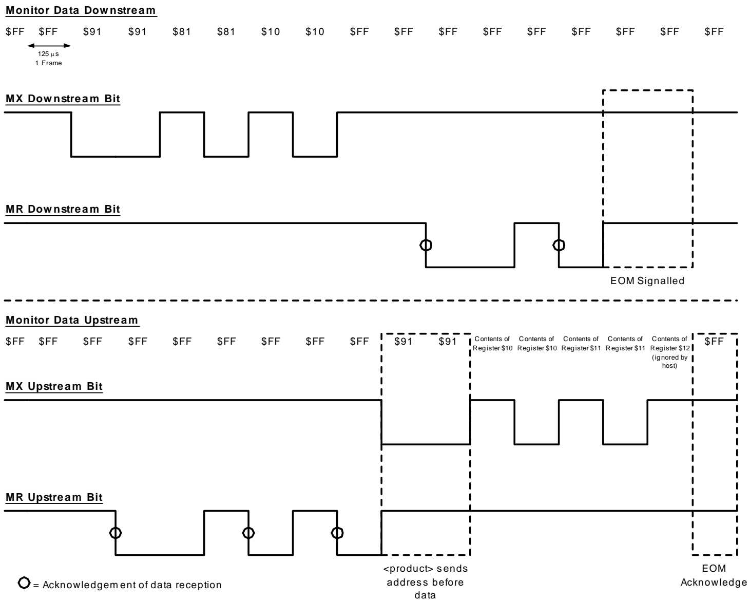
Figure 60. Example Read of Registers $10 and $11 in Channel 0 of the Dual ProSLIC
