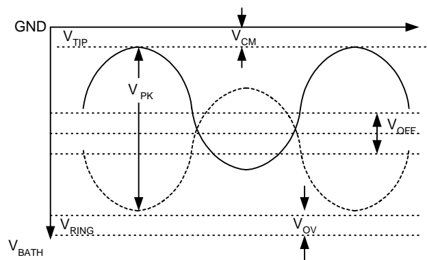
Figure 24. Balanced Ringing
