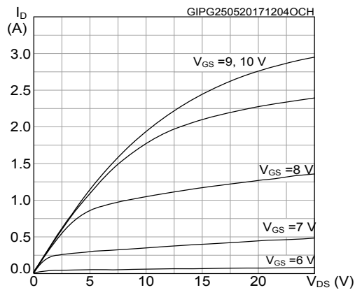
Figure 3. Output characteristics
