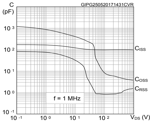
Figure 7. Capacitance variations
