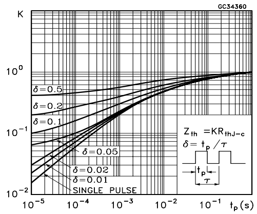
Figure 2. Thermal impedance
