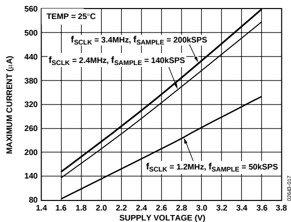
Figure 17. Maximum Current vs. Supply Voltage for Different SCLK Frequencies
