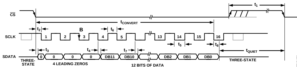
Figure 30. AD7466 Serial Interface Timing Diagram
