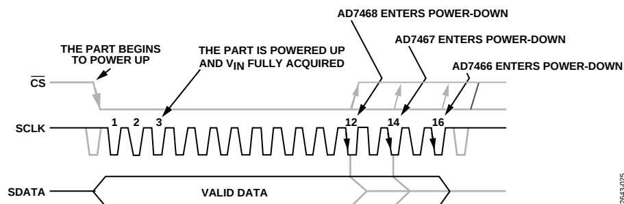
Figure 25. Normal Mode Operation
