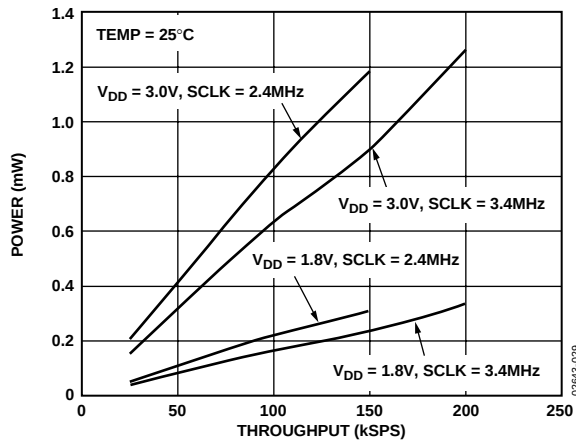
Figure 29. Power vs. Throughput Rate for Different SCLK and Supply Voltages
