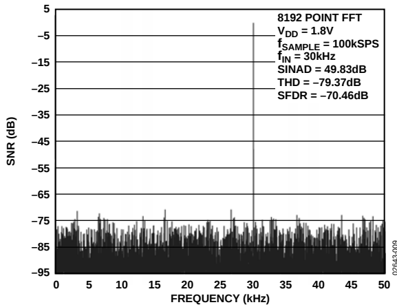
Figure 9. AD7468 Dynamic Performance at 100 kSPS
