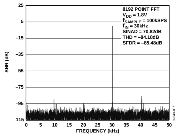
Figure 7. AD7466 Dynamic Performance at 100 kSPS
