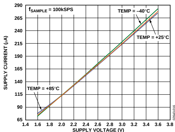
Figure 16. Supply Current vs. Supply Voltage, SCLK 3.4 MHz
