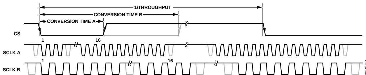
Figure 27. Conversion Time Comparison for Different SCLK Frequencies and a Fixed Throughput Rate
