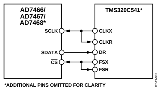
Figure 33. Interfacing to the TMS320C541
