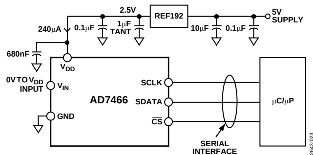
Figure 23. REF192 as Power Supply to AD7466
