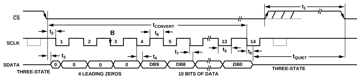
Figure 31. AD7467 Serial Interface Timing Diagram
