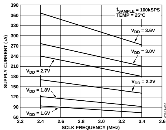
Figure 26. Supply Current vs. SCLK Frequency for a Fixed Throughput Rate and Different Supply Voltages
