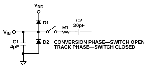
Figure 24. Equivalent Analog Input Circuit
