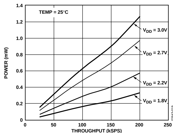
Figure 19. Power Consumption vs. Throughput Rate, SCLK 3.4 MHz
