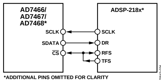
Figure 34. Interfacing to the ADSP-218x
