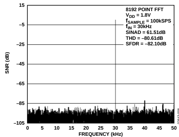
Figure 8. AD7467 Dynamic Performance at 100 kSPS
