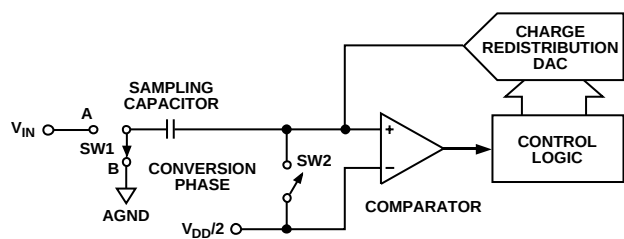
Figure 21. ADC Conversion Phase
