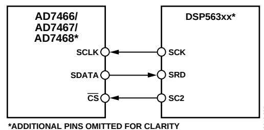
Figure 35. Interfacing to the DSP563xx
