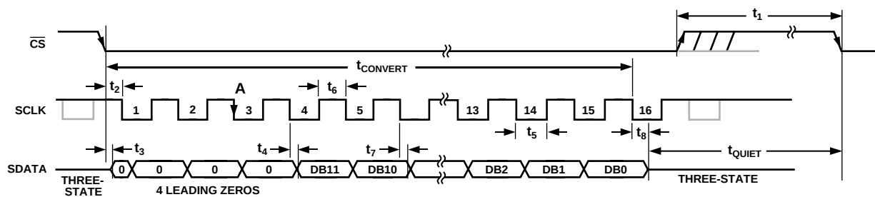
Figure 3. AD7466 Serial Interface Timing Diagram Example
