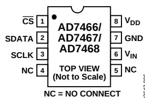
Figure 6. MSOP Pin Configuration
