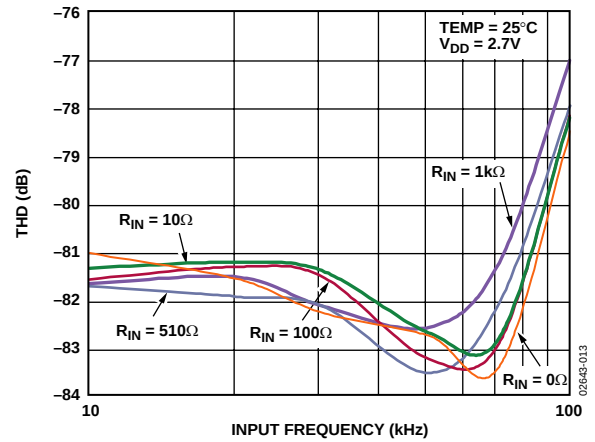
Figure 13. AD7466 THD vs. Analog Input Frequency for Various Source Impedances
