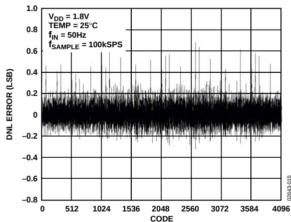
Figure 15. AD7466 DNL Performance
