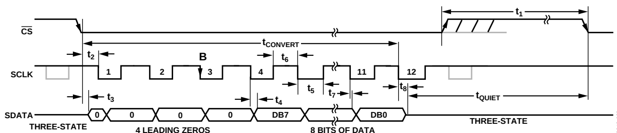
Figure 32. AD7468 Serial Interface Timing Diagram
