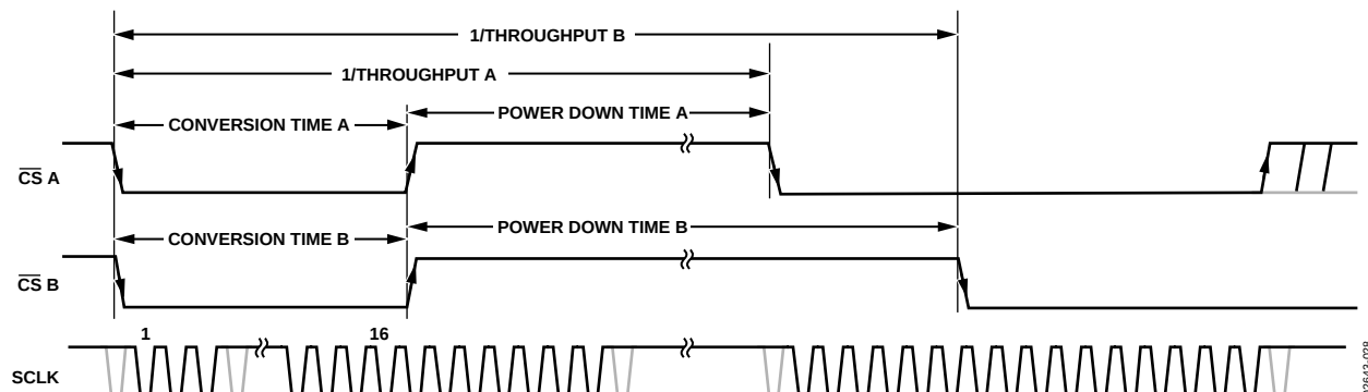
Figure 28. Conversion Time vs. Power-Down Time for a Fixed SCLK Frequency and Different Throughput Rates
