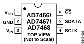
Figure 5. SOT-23 Pin Configuration
