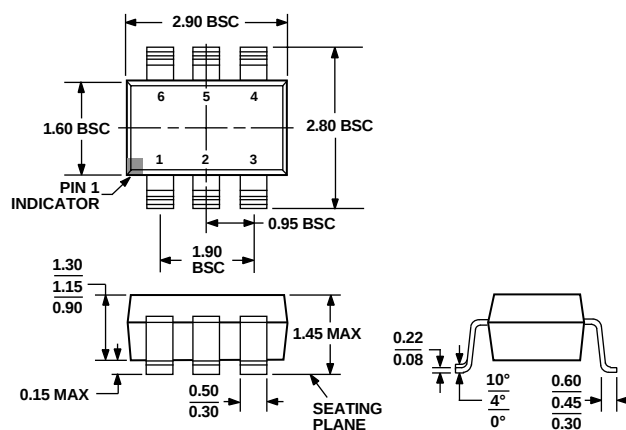
Figure 36. 6-Lead Small Outline Transistor Package [SOT-23] (RT-6) Dimensions shown in millimeters
