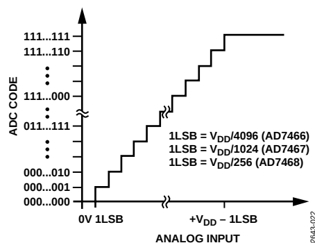
Figure 22. AD7466/AD7467/AD7468 Transfer Characteristics
