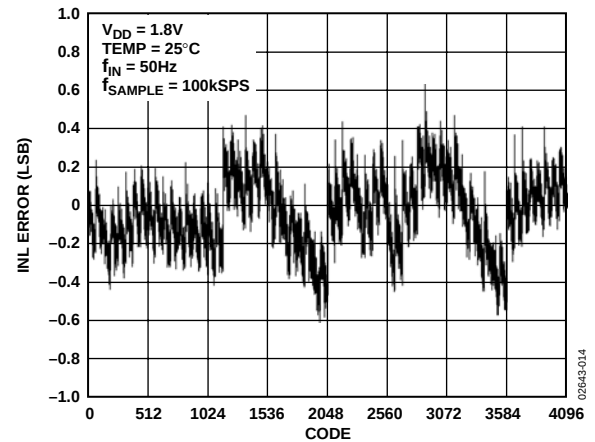
Figure 14. AD7466 INL Performance
