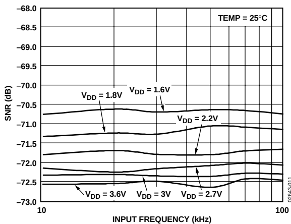
Figure 11. AD7466 SNR vs. Analog Input Frequency at 100 kSPS for Various Supply Voltages
