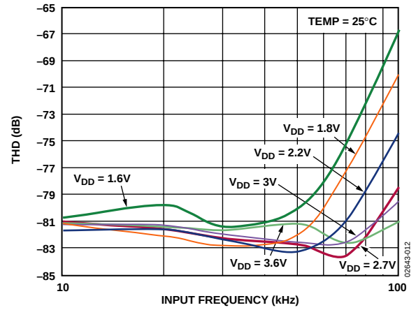
Figure 12. AD7466 THD vs. Analog Input Frequency at 100 kSPS for Various Supply Voltages
