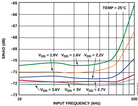
Figure 10. AD7466 SINAD vs. Analog Input Frequency at 100 kSPS for Various Supply Voltages
