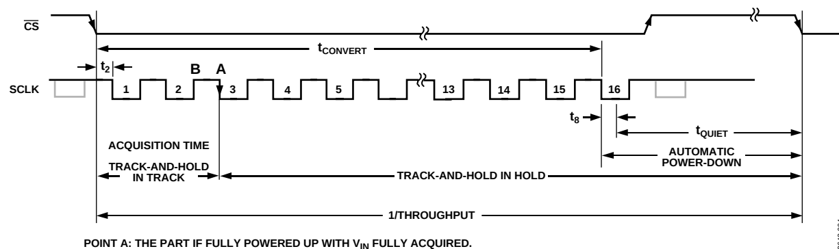
Figure 4. AD7466 Serial Interface Timing Diagram Example
