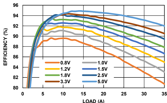
FIGURE 7. V_{OUT} POWER STAGE EFFICIENCY ( V_{IN} = 12V ; 500kHz; L_{OUT} = 0.18\mu H/0.17m\Omega/FP1008-180-R ; INCLUDE INDUCTOR AND ISL99135B LOSSES)
