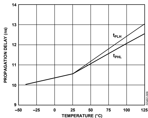
Figure 9. Typical Propagation Delays vs. Temperature, 5 V/3 V Operation
