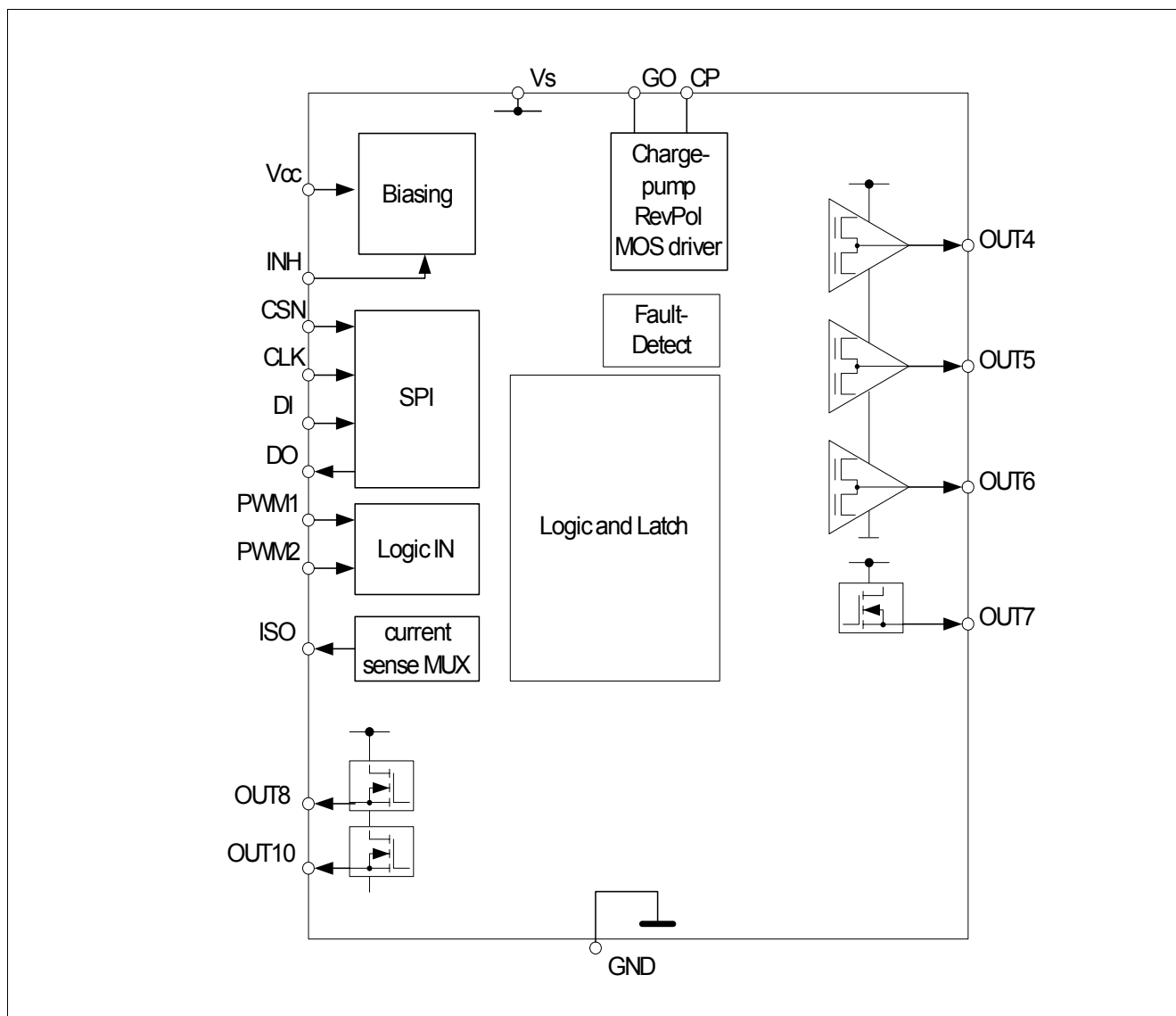
Figure 1 Block Diagram
