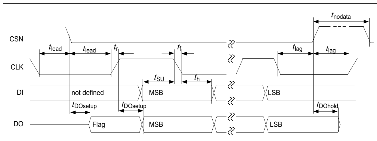
Figure 7 Timing Diagram
