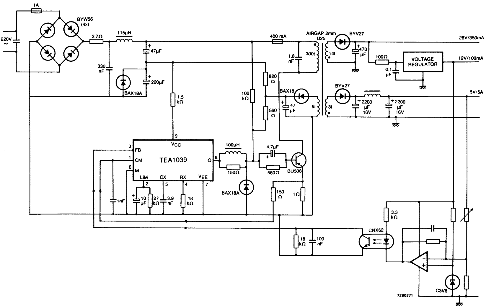
Fig.9 Typical application of the TEA1039 in a variable-frequency flyback converter switched-mode power supply. An optocoupler CNX62 is used for voltage separation.
