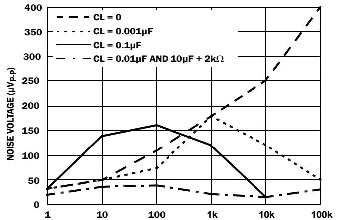
FIGURE 117. NOISE REDUCTION
