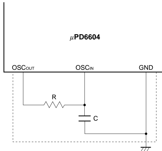
Figure 8-1. System Clock
