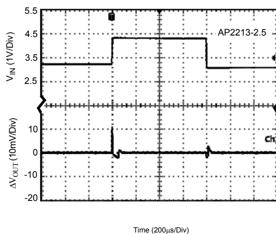
Figure 11. Line Transient (Conditions: V_{IN} = 3.4 to 4.4V , V_{EN} = 2V , I_{OUT} = 100\mu A , C_{BYF} = 100pF , C_{OUT} = 2.2\mu F )
