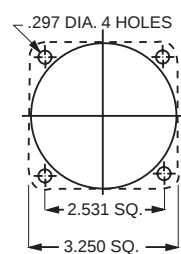
PANEL MOUNTING HOLES
