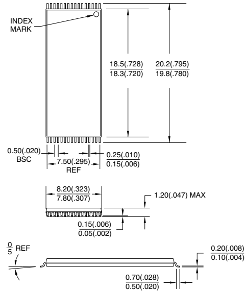
32T, 32-lead, Plastic Thin Small Outline Package (TSOP) Dimensions in Millimeters and (Inches)* JEDEC OUTLINE MO-142 BA
