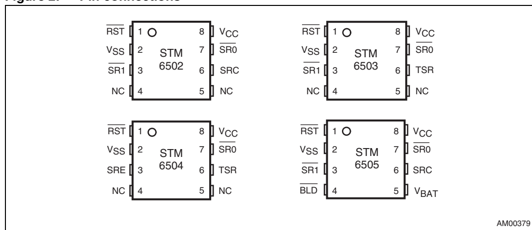
Figure 2. Pin connections
