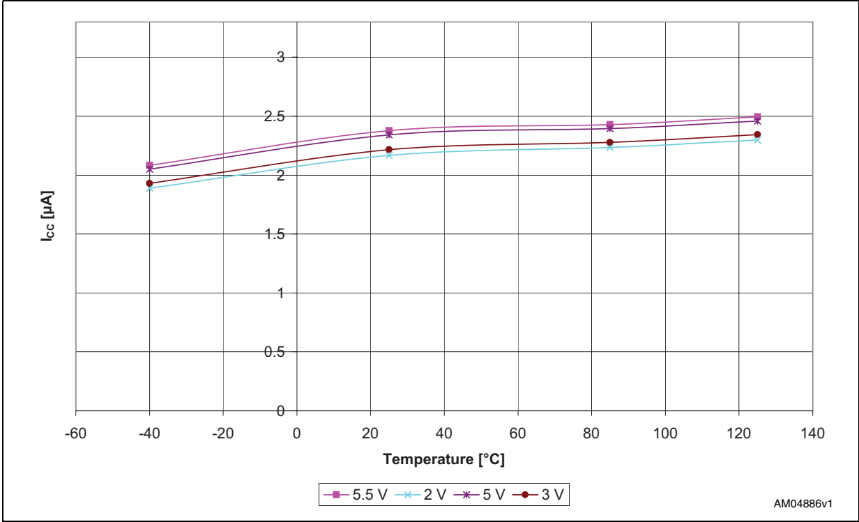
Figure 10. Supply current ( I_{CC} ) vs. temperature (STM6505)
