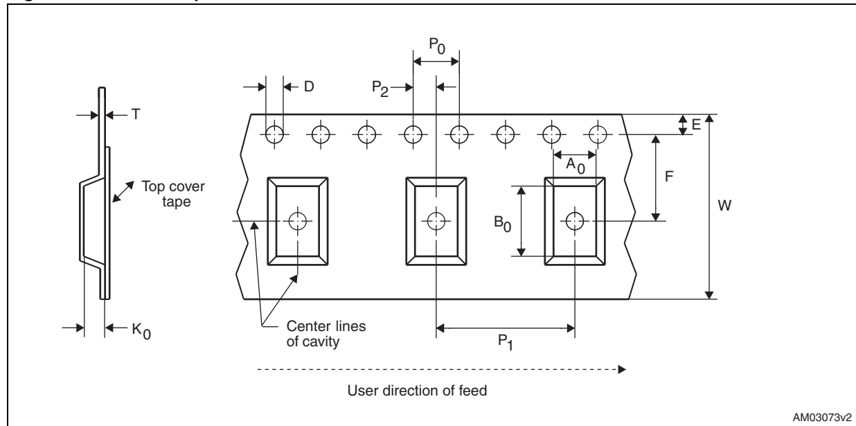
Figure 17. Carrier tape
