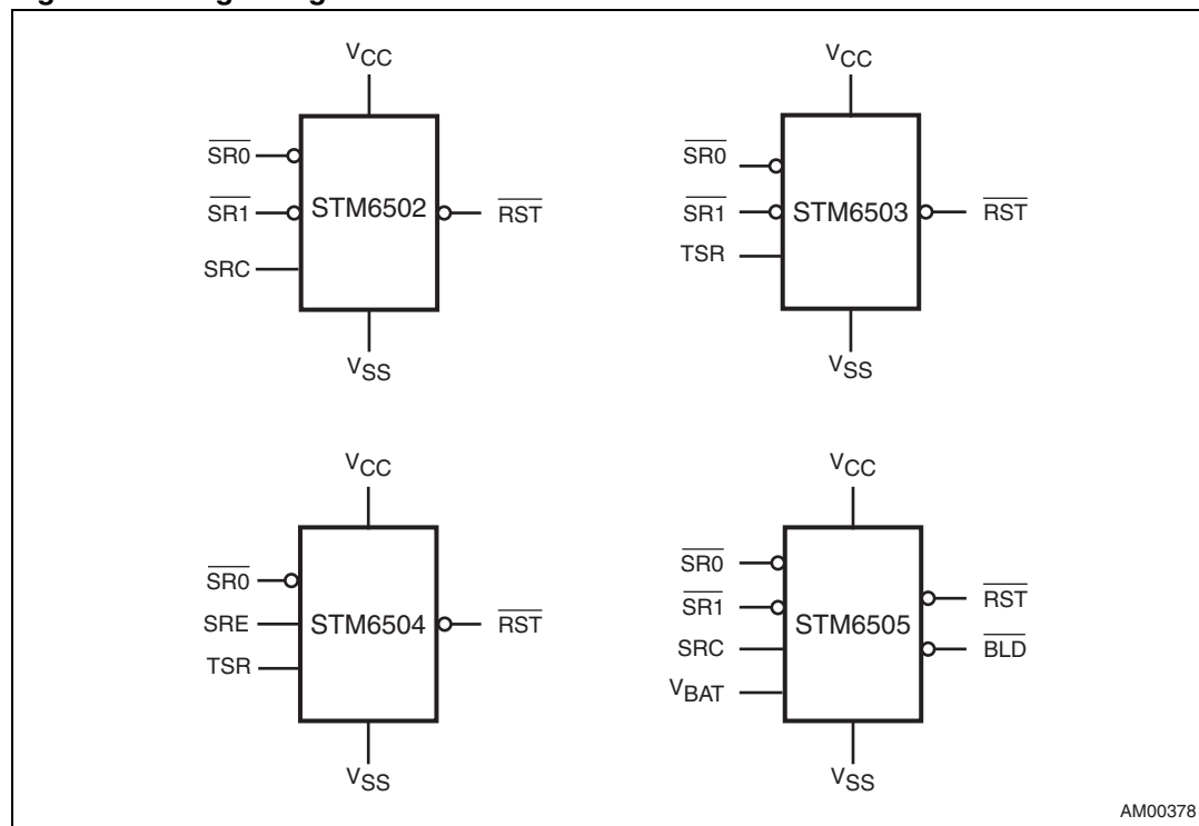
Figure 1. Logic diagrams
