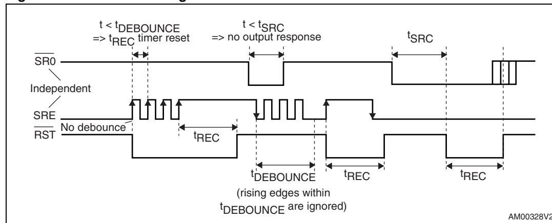
Figure 8. STM6504 timing
