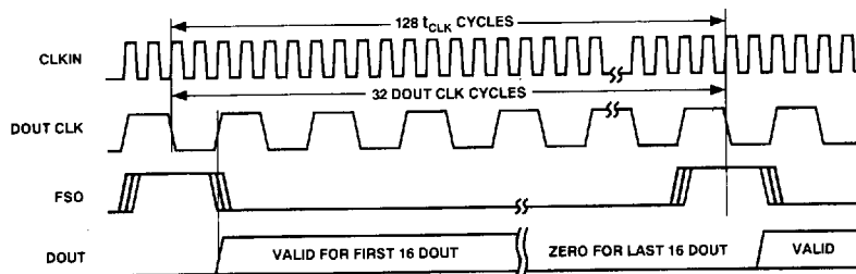
Figure 14b. Mode A Timing
