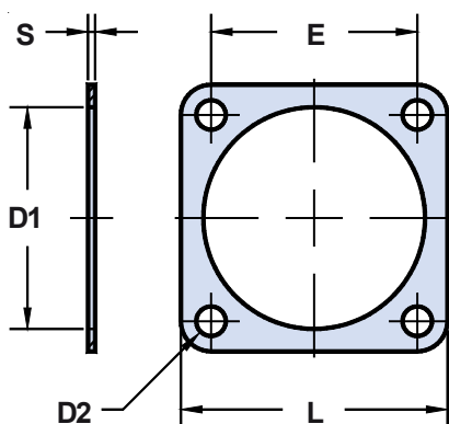
DA1 Non-Conductive
