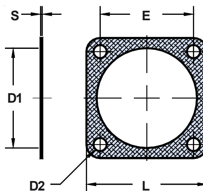
DA2 Conductive
