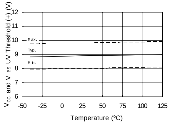
Figure 18. V CC and V BS Undervoltage Threshold (+) vs. Temperature
