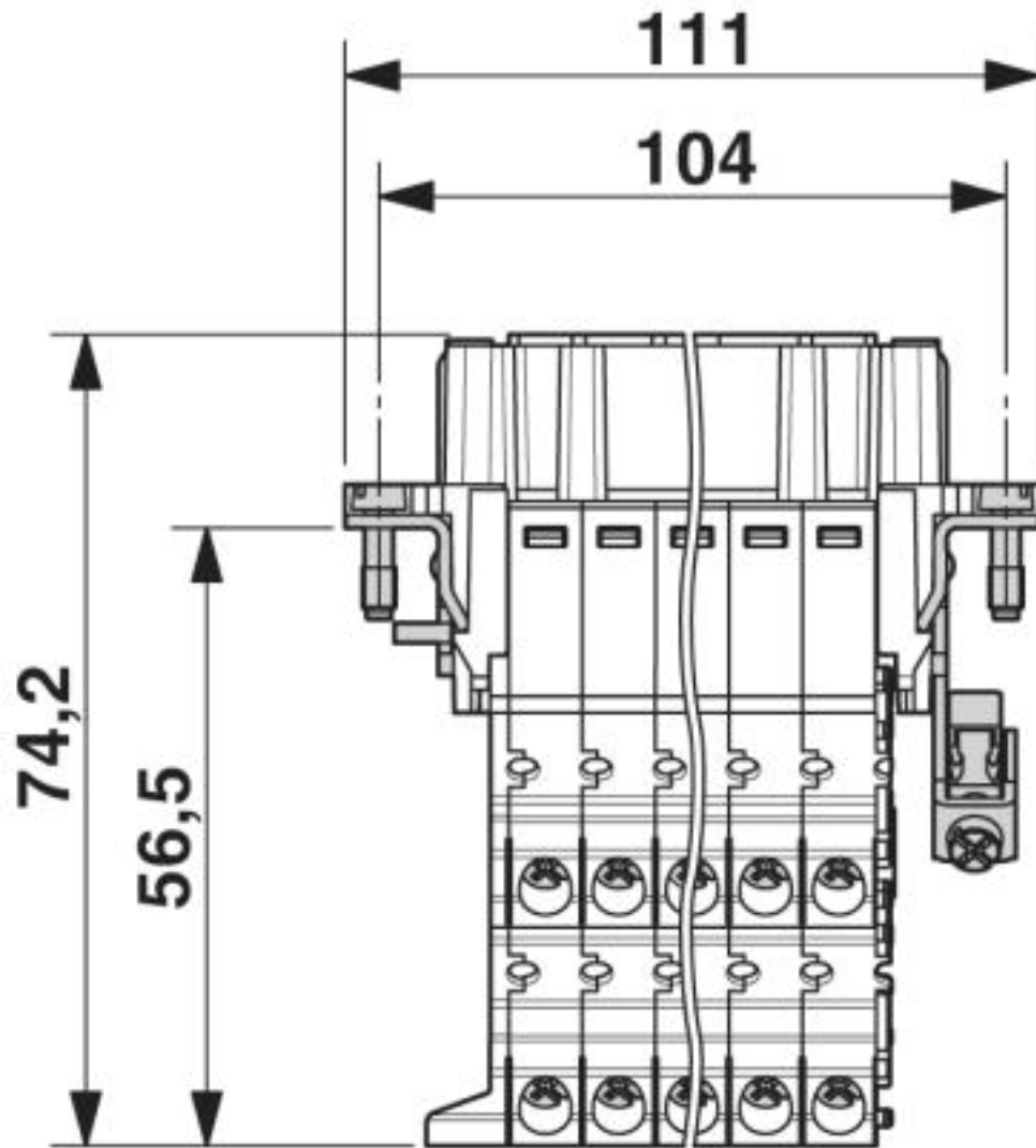
Dimensional drawing
