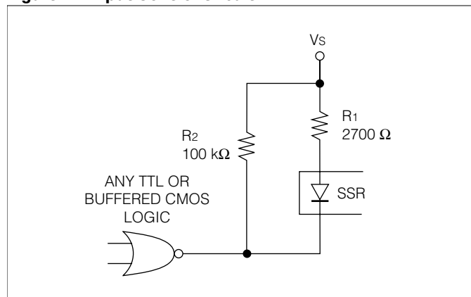
Figure 22. Input Control Circuit
