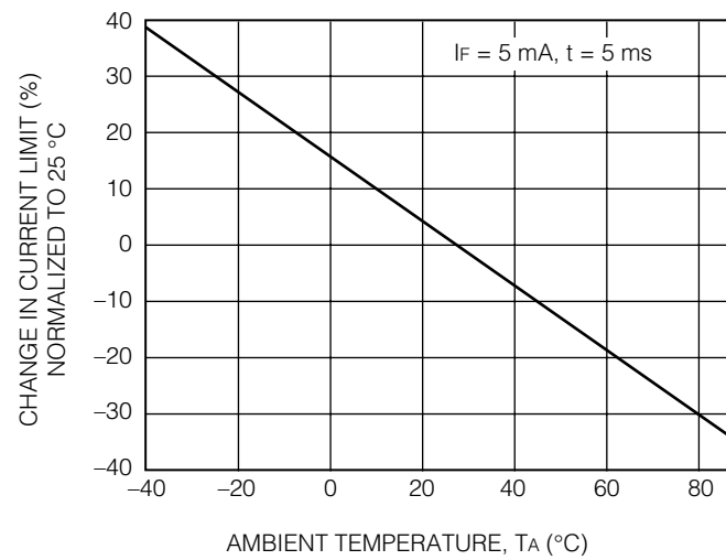
Figure 8. Current Limit vs. Temperature
