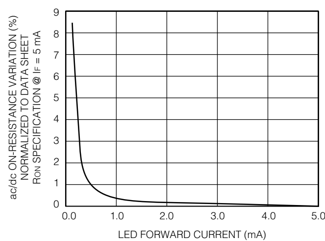
Figure 9. Variation in ON-Resistance vs. LED Current
