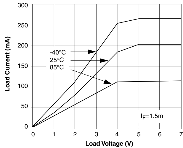
Figure 7. Load Current vs. Load Voltage
