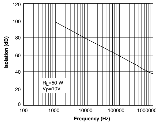
Figure 11. Output Isolation
