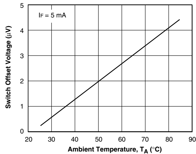
Figure 16. Switch Offset Voltage vs. Temperature
