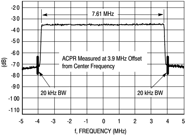
Figure 15. 8K Mode DVB-T OFDM Spectrum
