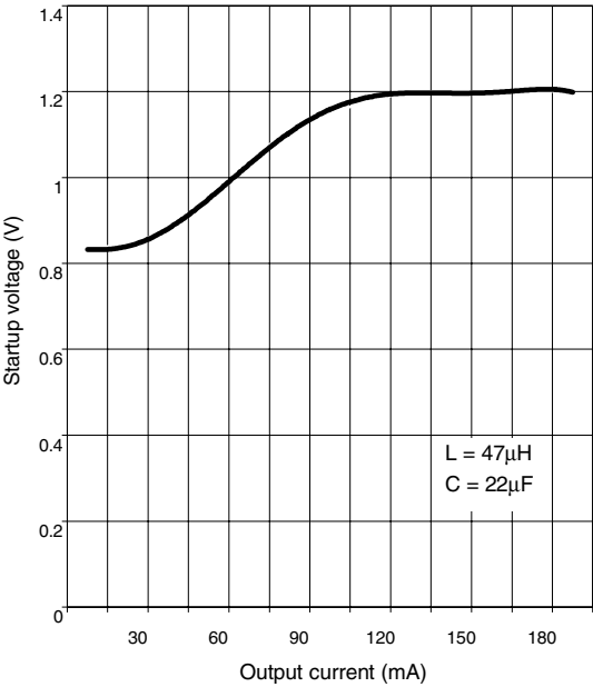
Figure 5. Startup Voltage vs Output Current
