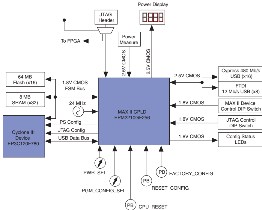
Figure 2–3. MAX II Device's Block Diagram
