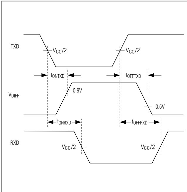
Figure 1. Timing Diagram
