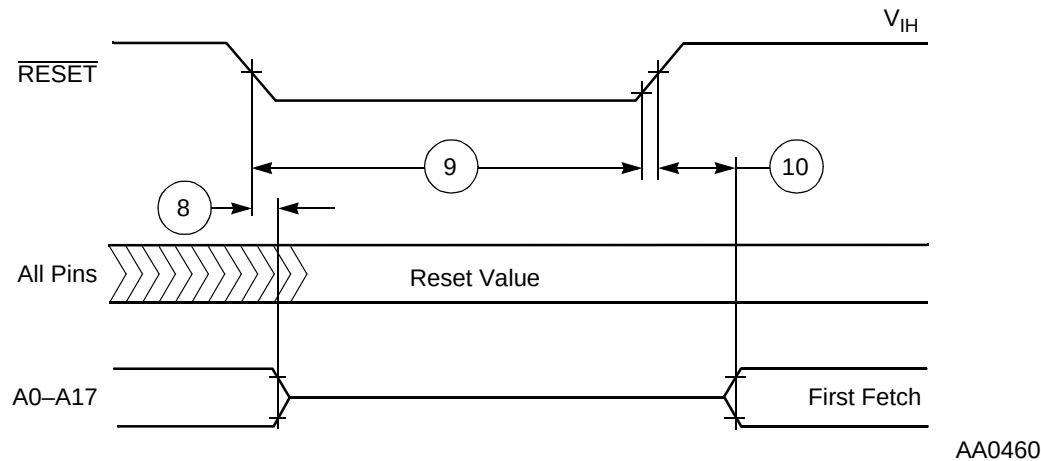
Figure 3-2 Reset Timing
