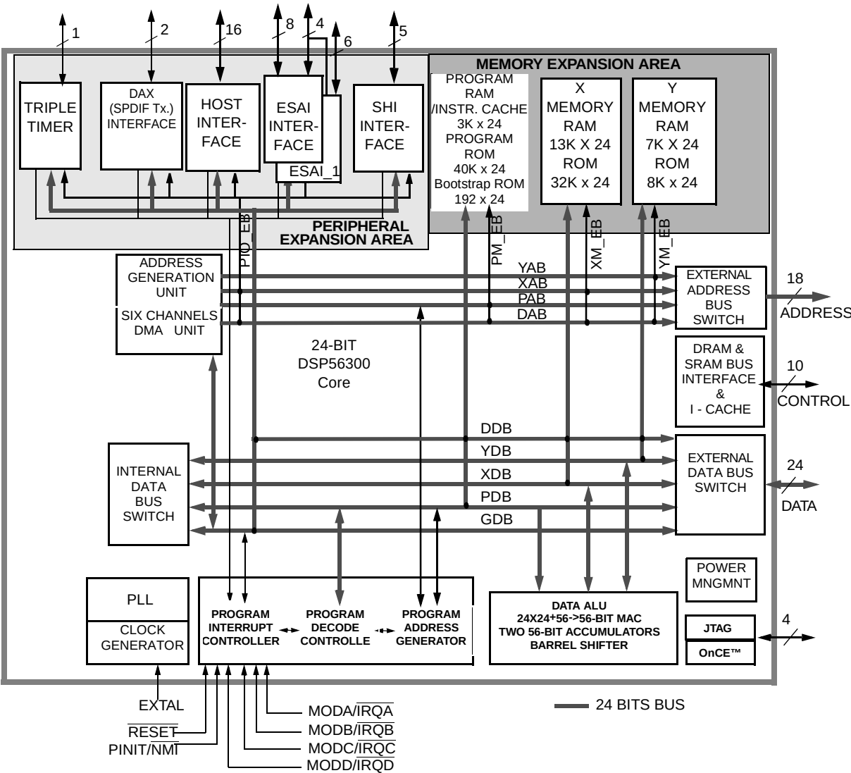
Figure 1-1 DSP56367 Block Diagram
