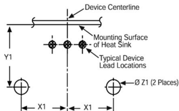
Mounting Details:
