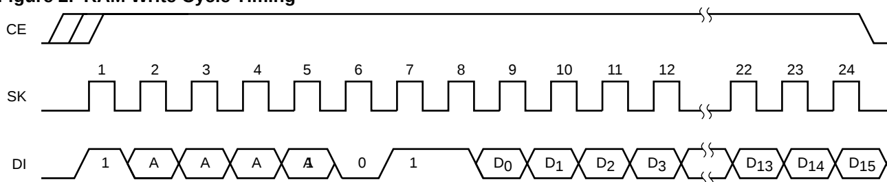
Figure 2. RAM Write Cycle Timing
