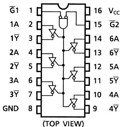
TC74HC366A
