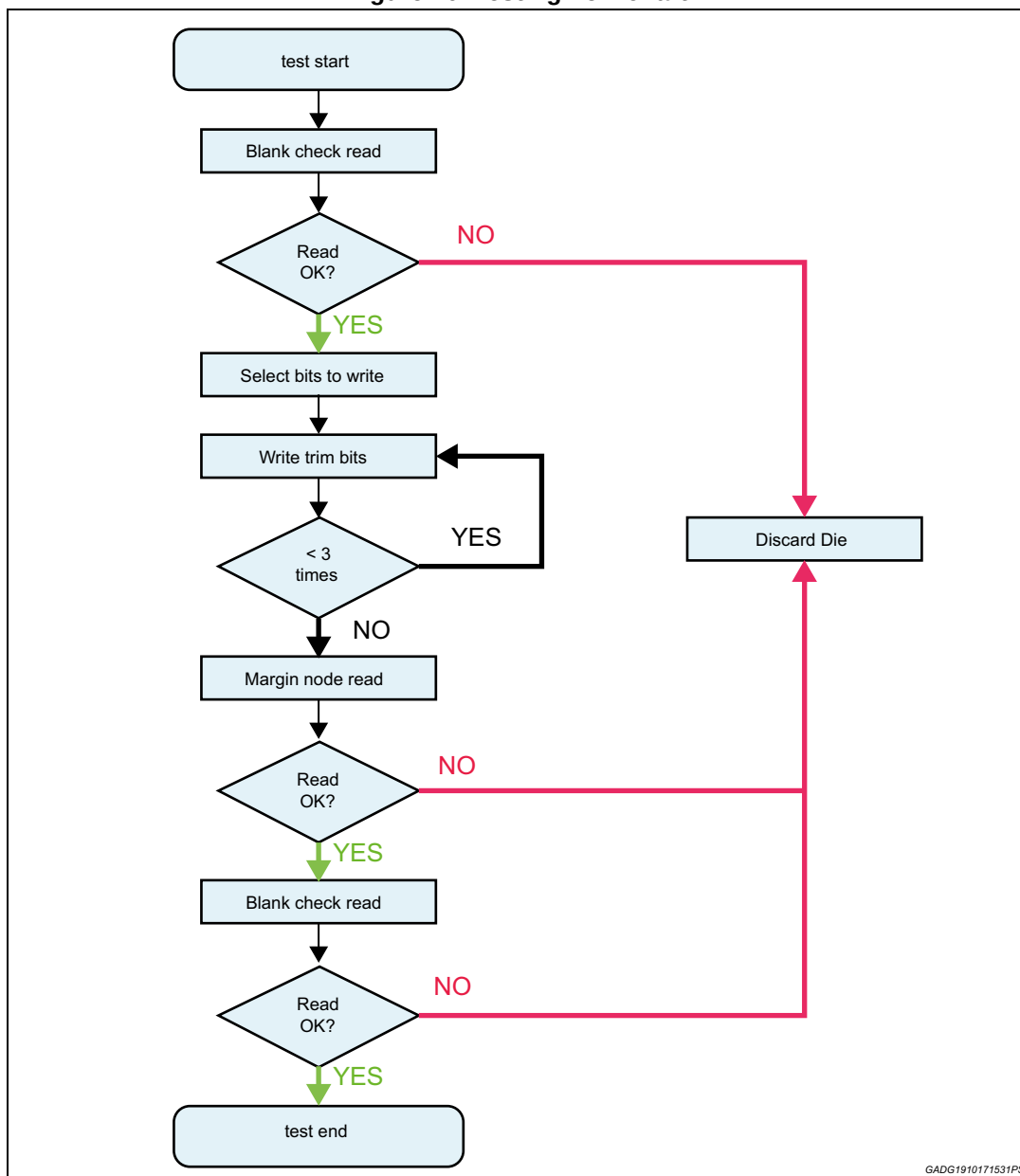
Figure 10. Testing flow chart
