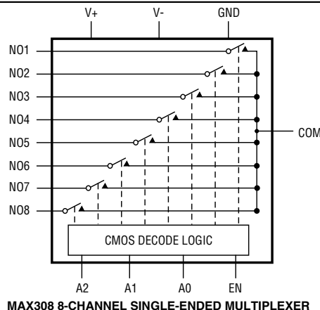
MAX308 8-CHANNEL SINGLE-ENDED MULTIPLEXER
