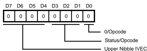
Figure 63. IVEC Register (Z180 MPU, Address xxFCh)
