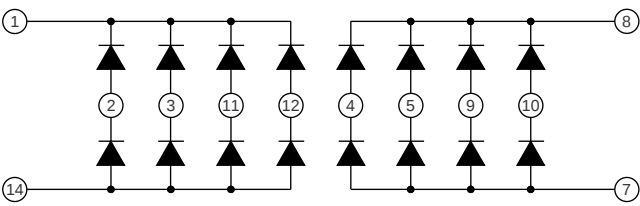
DUAL 8 DIODE ARRAY NC Pins 6 & 13
