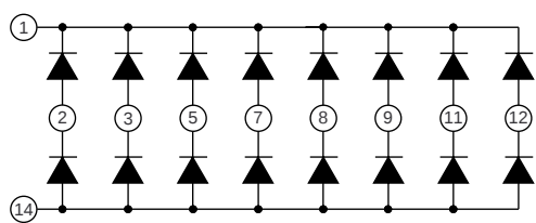
16 DIODE ARRAY NC Pins 4, 6, 10 & 13
