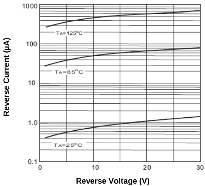
Fig.3-Typical Reverse Characteristics
