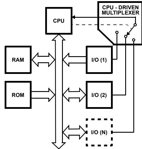
FIGURE 2. POLLED METHOD
