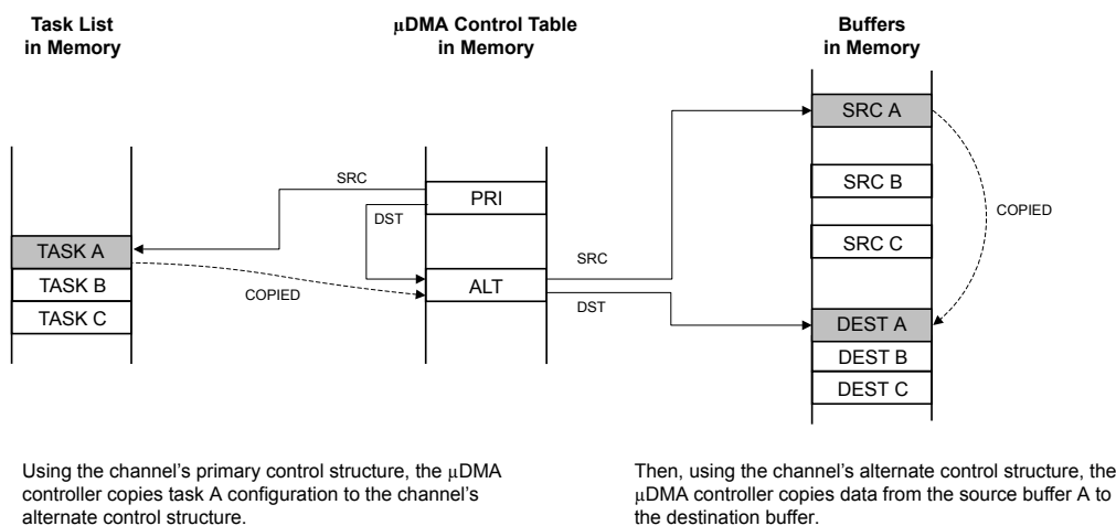
Figure 8-4. Memory Scatter-Gather, \mu DMA Copy Sequence
