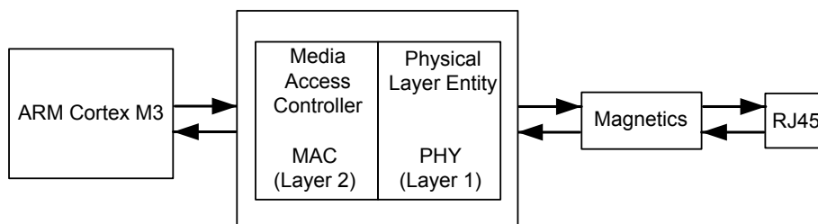
Figure 19-1. Ethernet Controller
