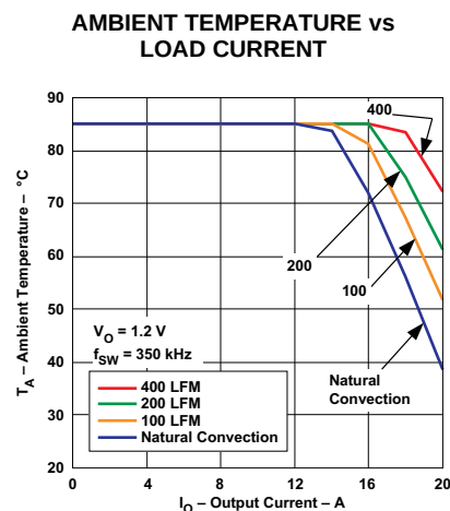
Figure 15. Safe Operating Area
