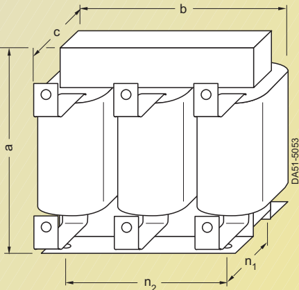
Line commutating choke for inverter frame sizes FX and GX
