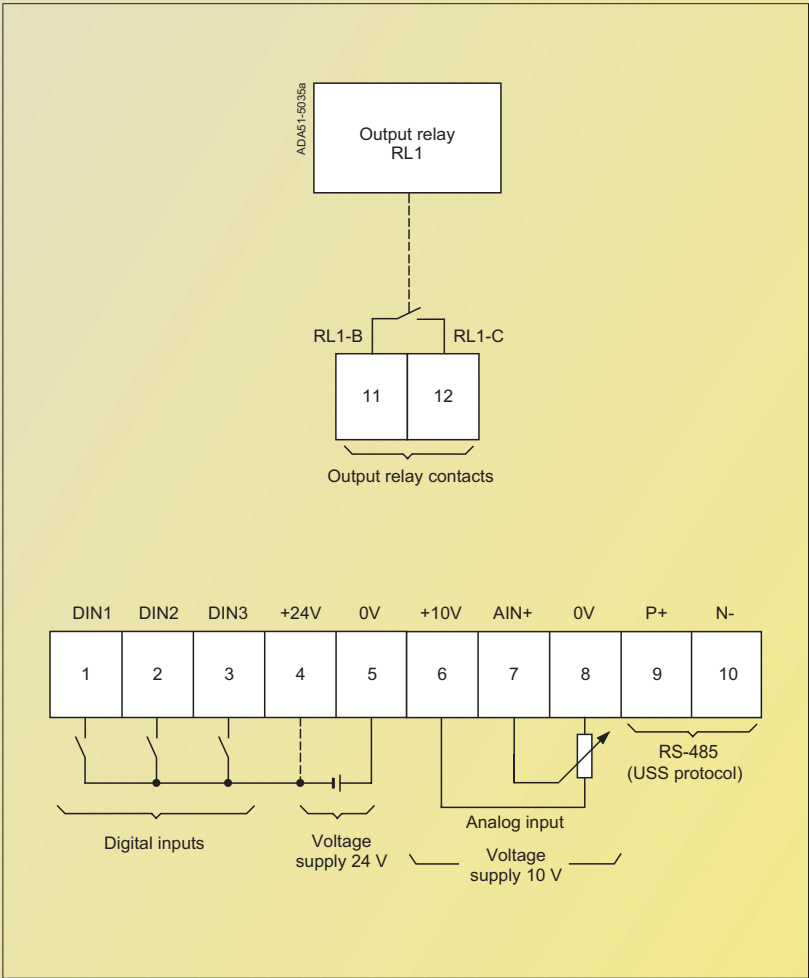
View A
