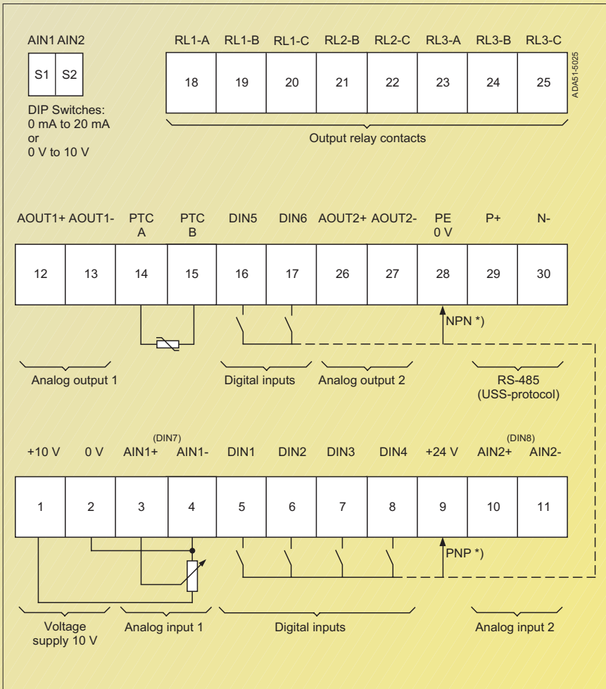
View A
