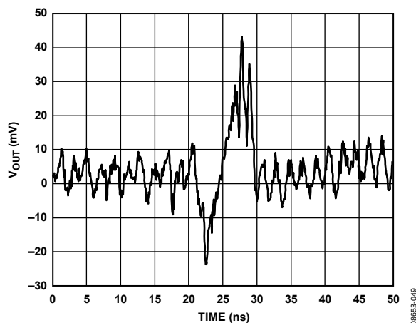
Figure 46. ADV3227 Switching Glitch
