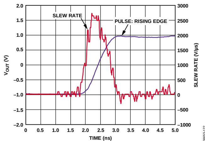
Figure 22. ADV3227 Rising Edge Slew Rate
