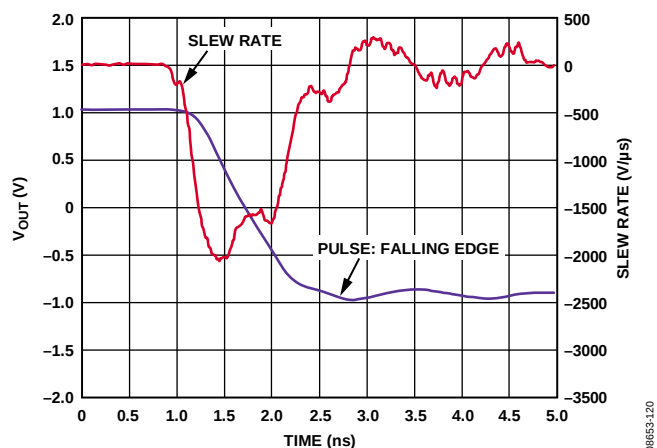
Figure 20. ADV3226 Falling Edge Slew Rate
