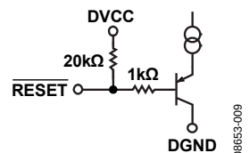
Figure 63. Reset Input
