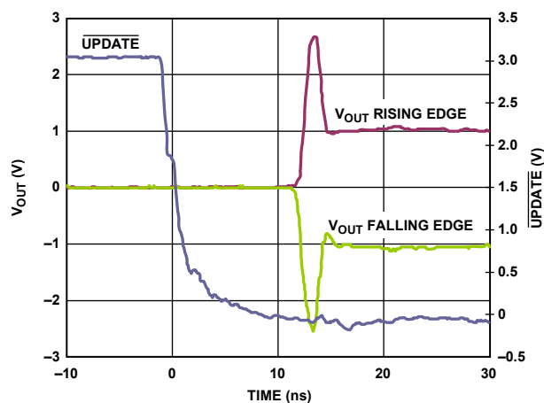
Figure 44. ADV3226 Enable Time
