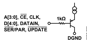
Figure 61. Logic Input
