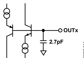
Figure 62. Analog Output Disabled
