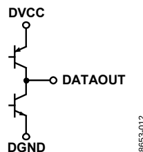
Figure 64. Logic Output
