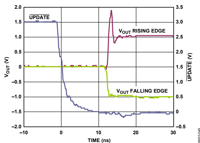
Figure 47. ADV3227 Enable Time
