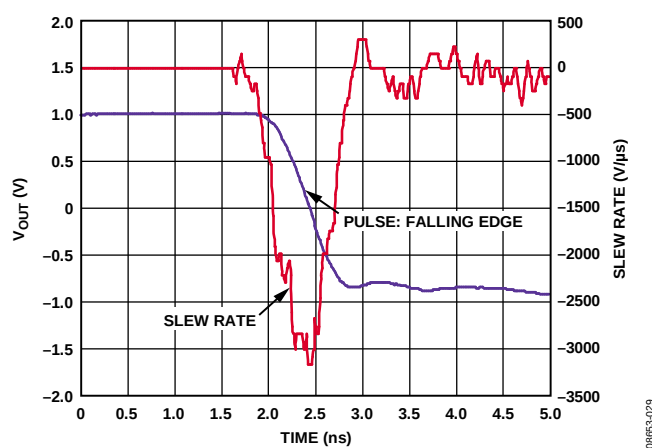
Figure 23. ADV3227 Falling Edge Slew Rate
